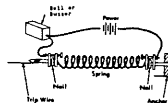
Figure 385 Tension Release Device Booby Trap
