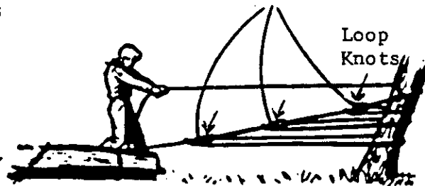
Figure 198 Lumberjack's pulley
