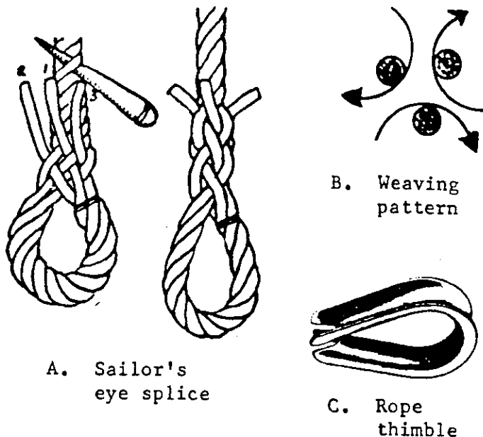
Figure 170 Sailor's Eye Splice
