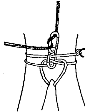
Figure 222-B The Rappel Rope Snaplink Attachment for the Seat-Hip Rappel
