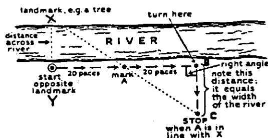
Figure 433 Determining the Width of a River
