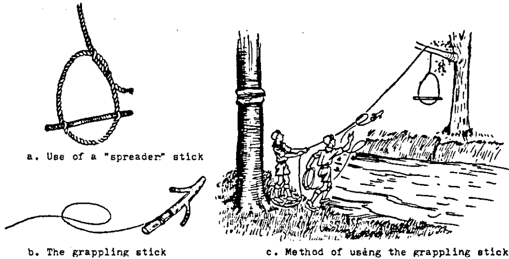
Figure 254 Using a Grappling Stick to Get a First Line Across for a One Rope Bridge
